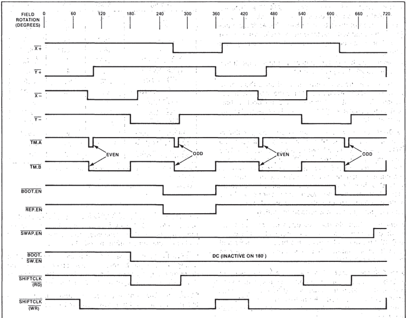
Figure 4. 7220 BMC Timing Diagram
