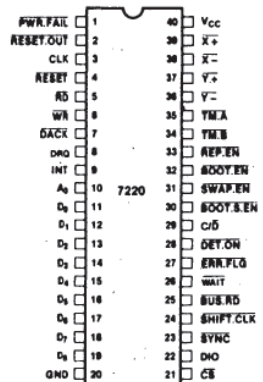
Figure 2. 7220 Pin Configuration
