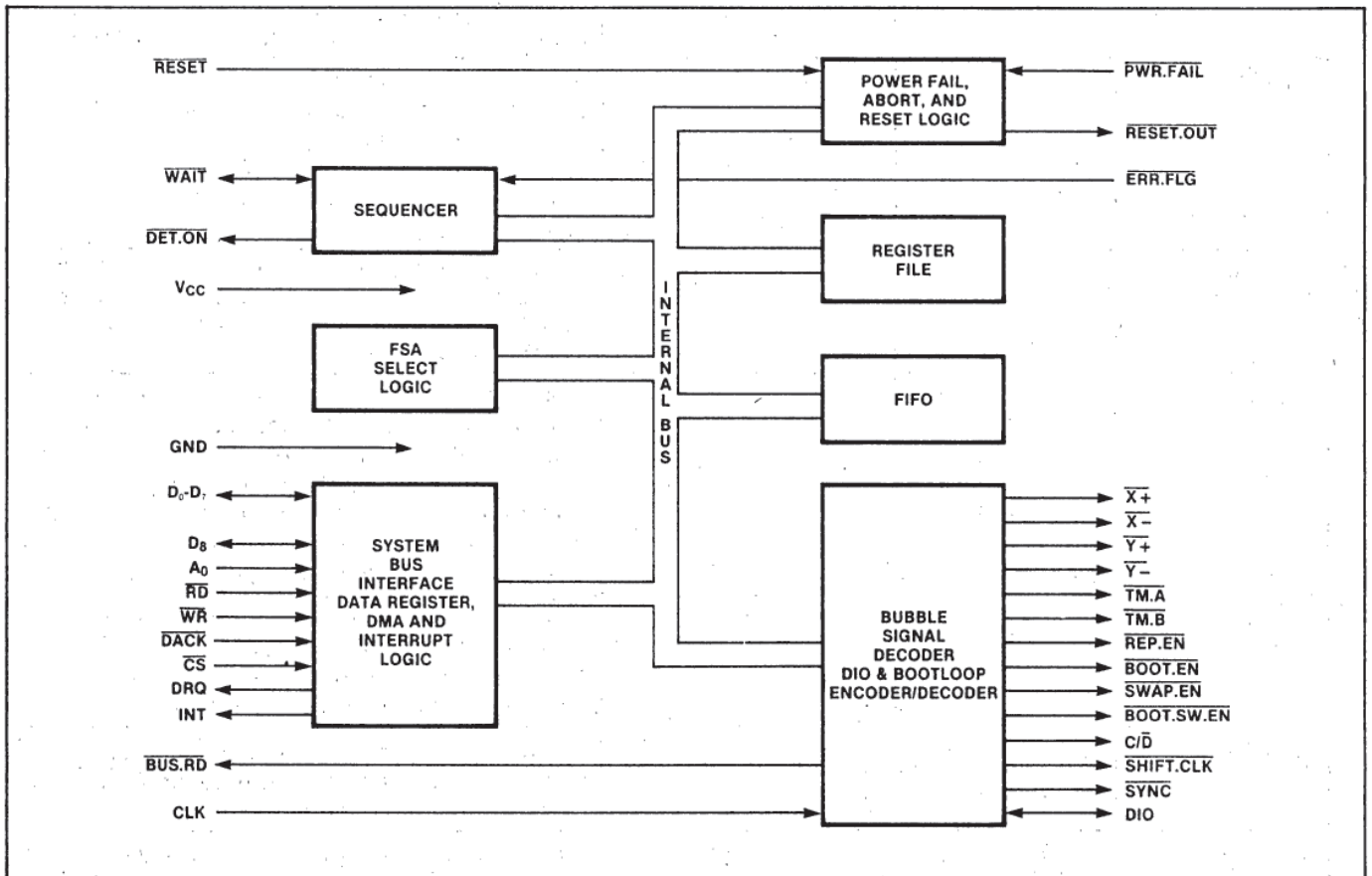
Figure 3. 7220 Bubble Memory Controller (BMC), Block Diagram
